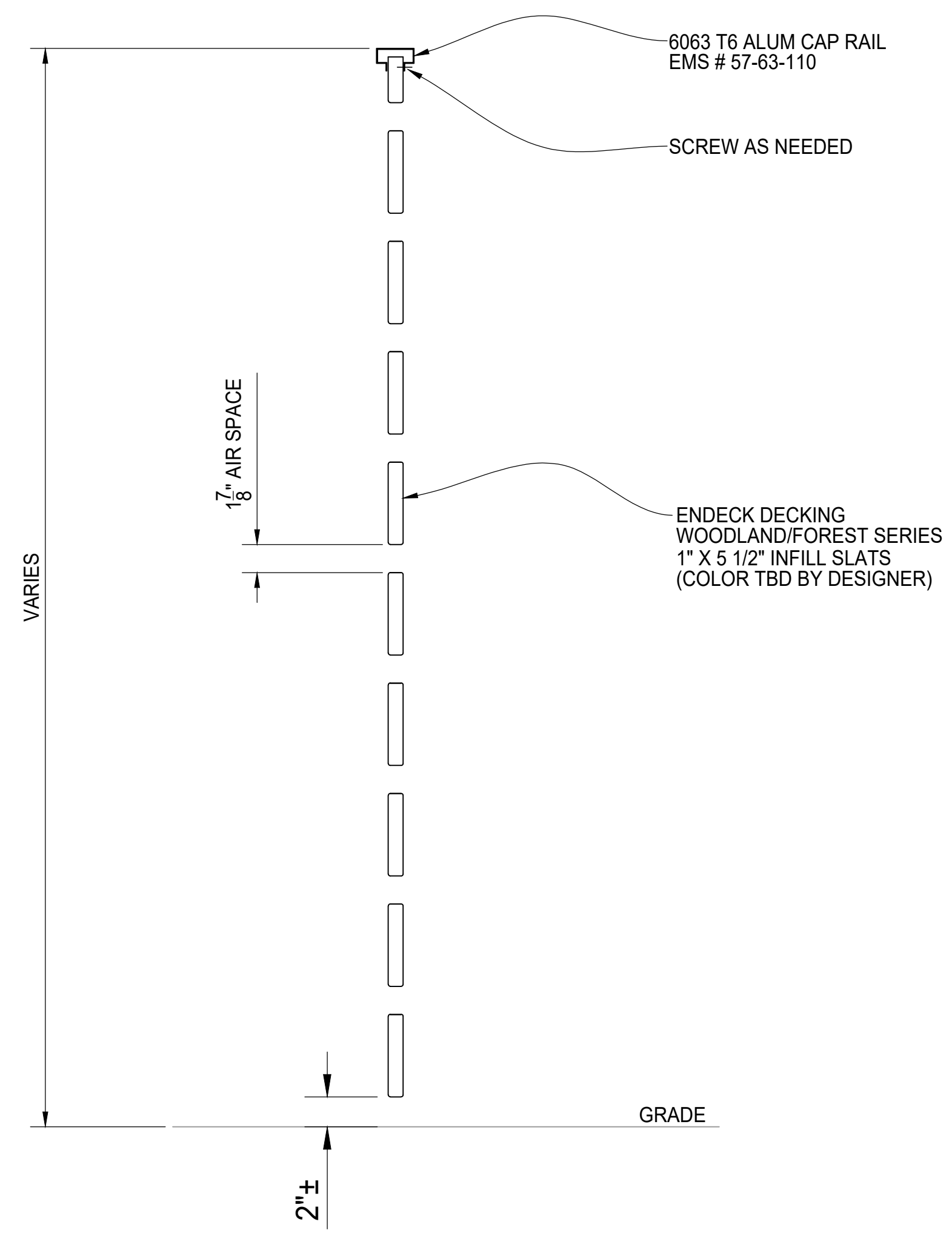
SIDE VIEW PANEL SECTION
