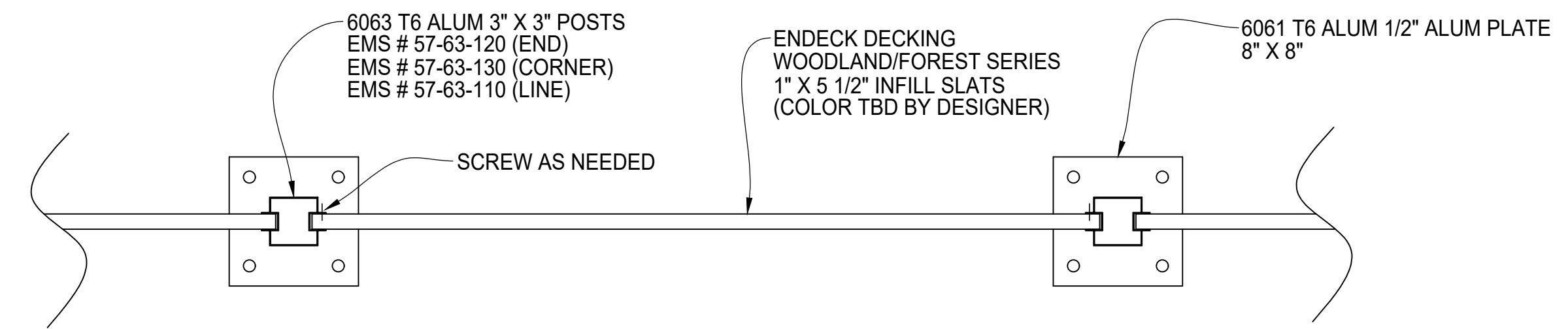
TOP VIEW PANEL SECTION
