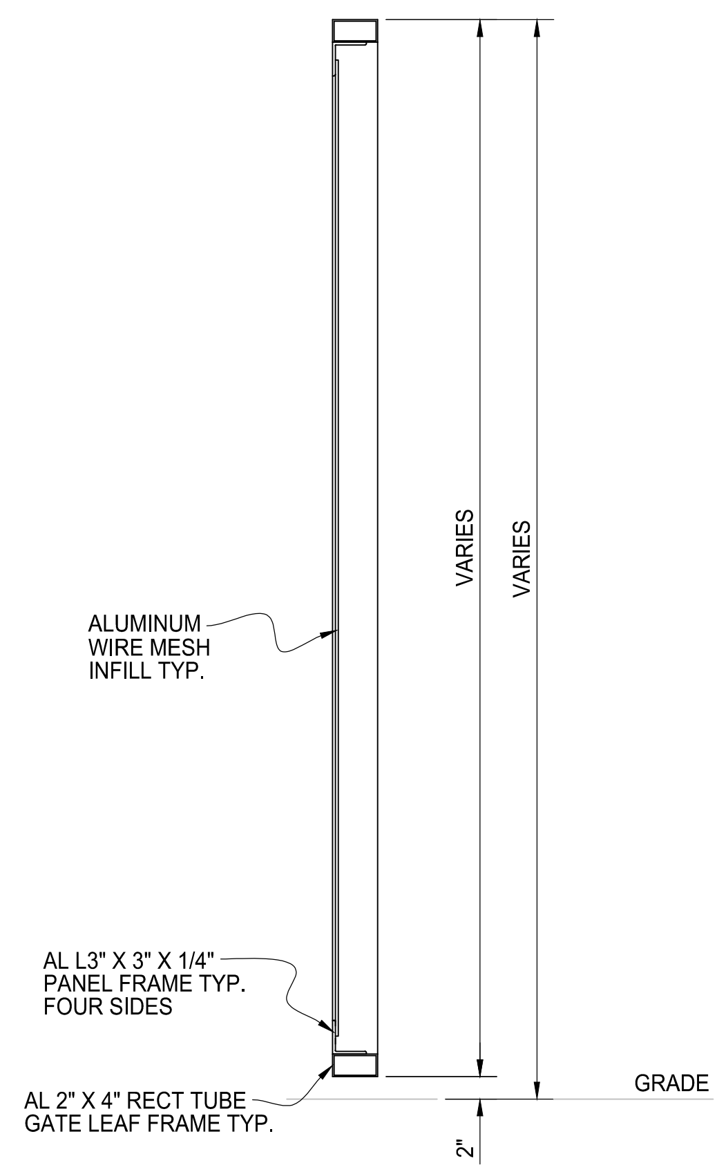
TYPICAL GATE SECTION ALUM 2" X 2" SQUARE .25" WIRE WEAVE MESH
