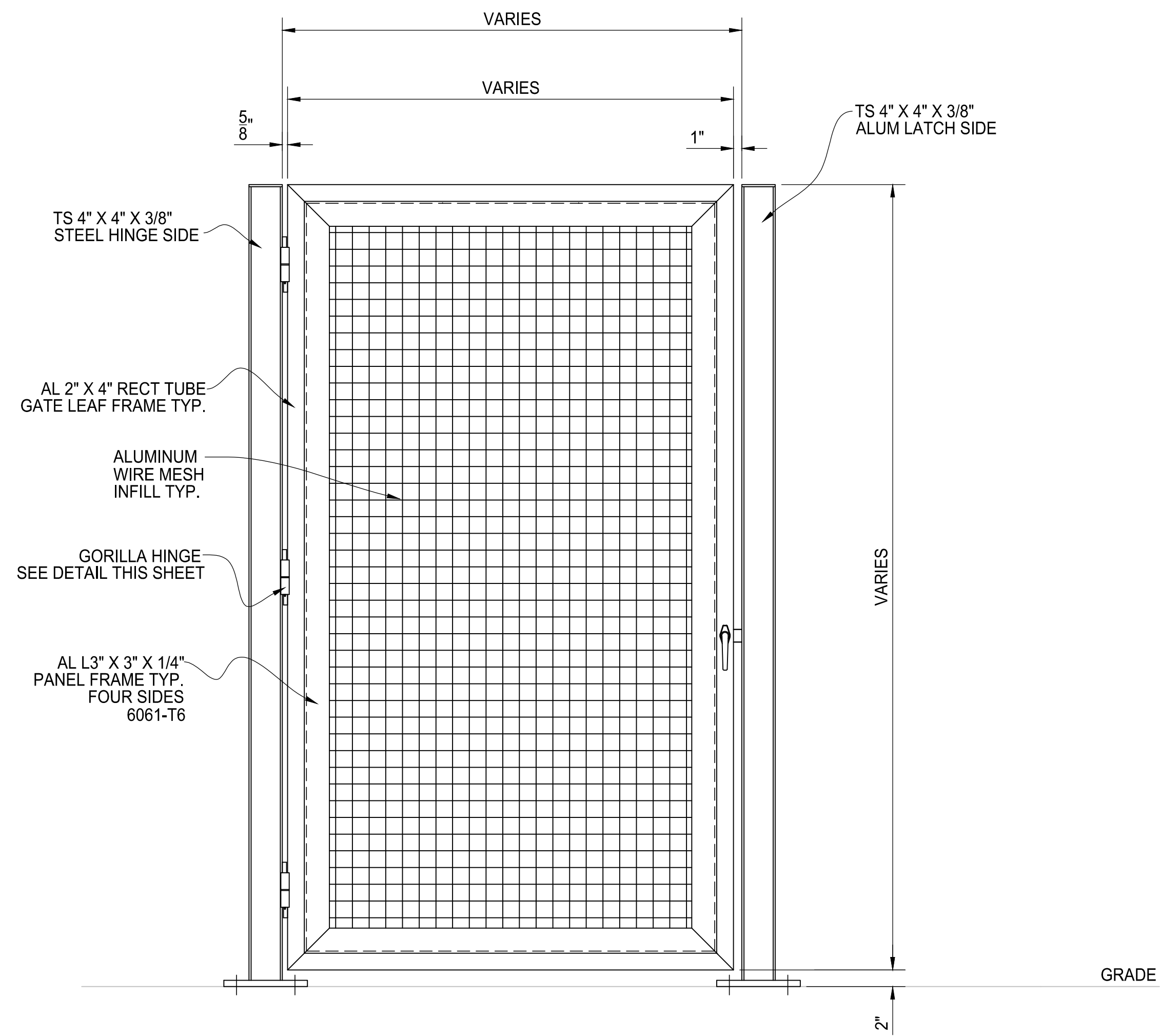
ELEVATION VIEW
