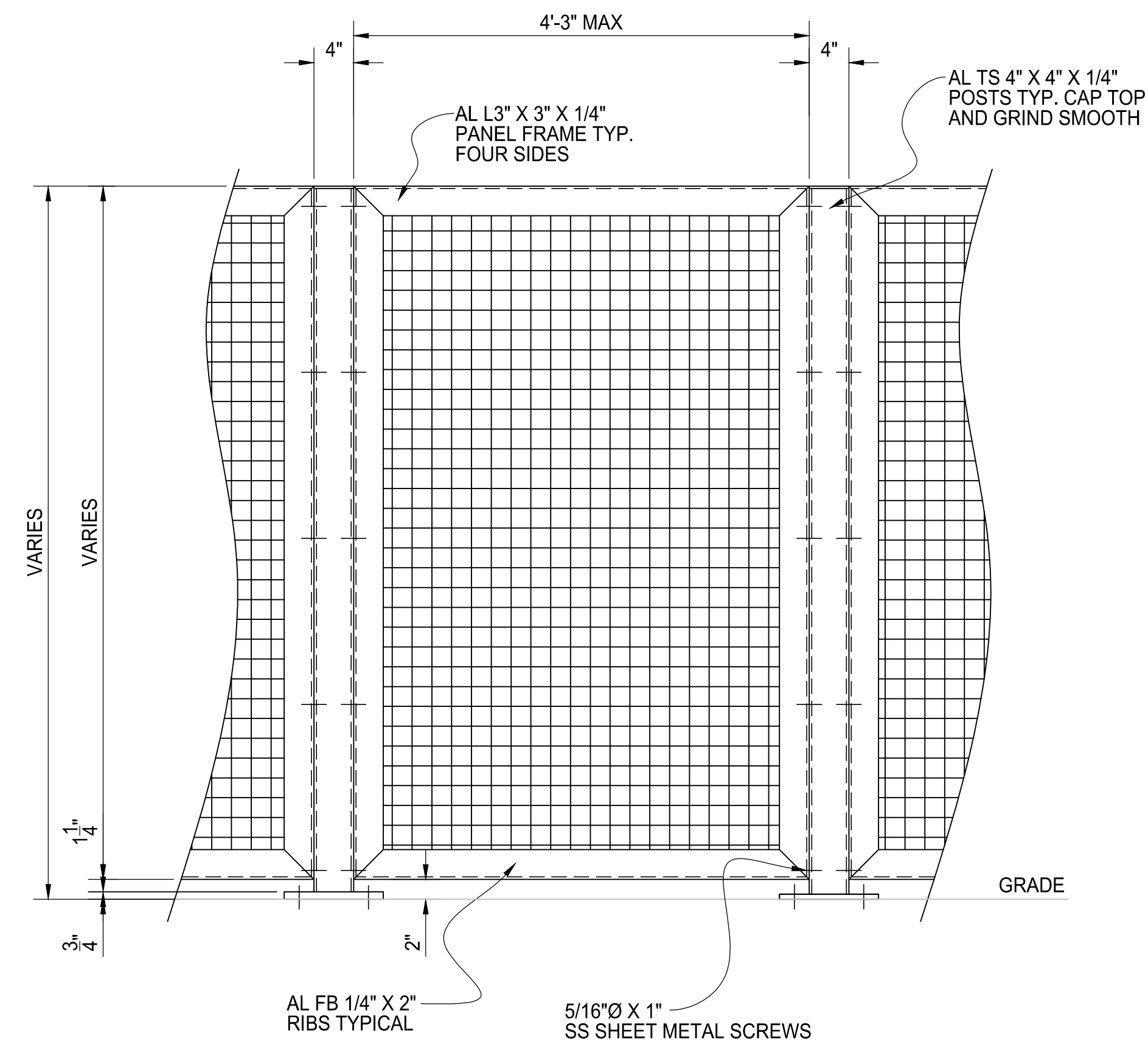
ELEVATION VIEW
