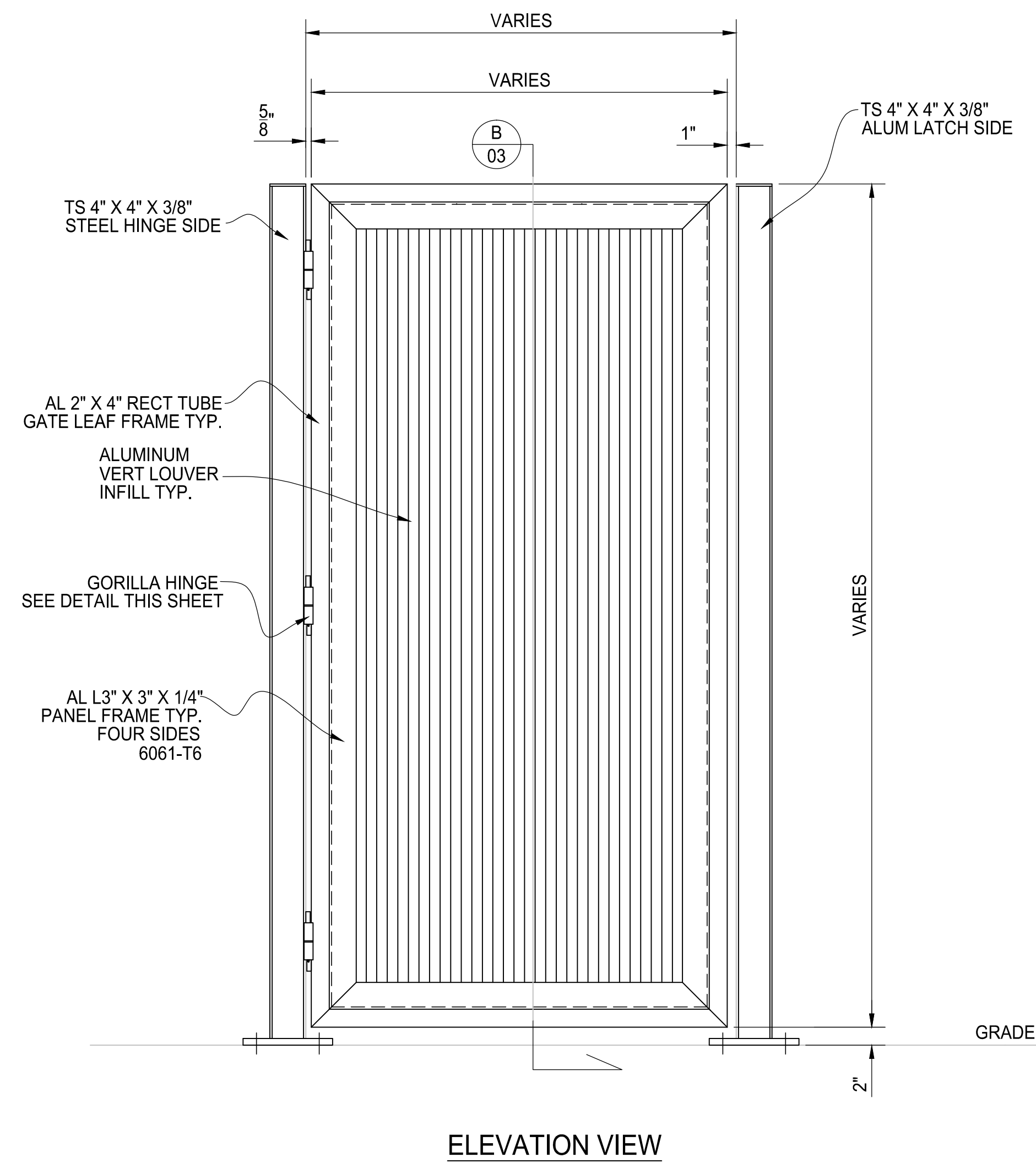
SINGLE SWING GATE ASSEMBLY ALUM 1 3/4\"/>
