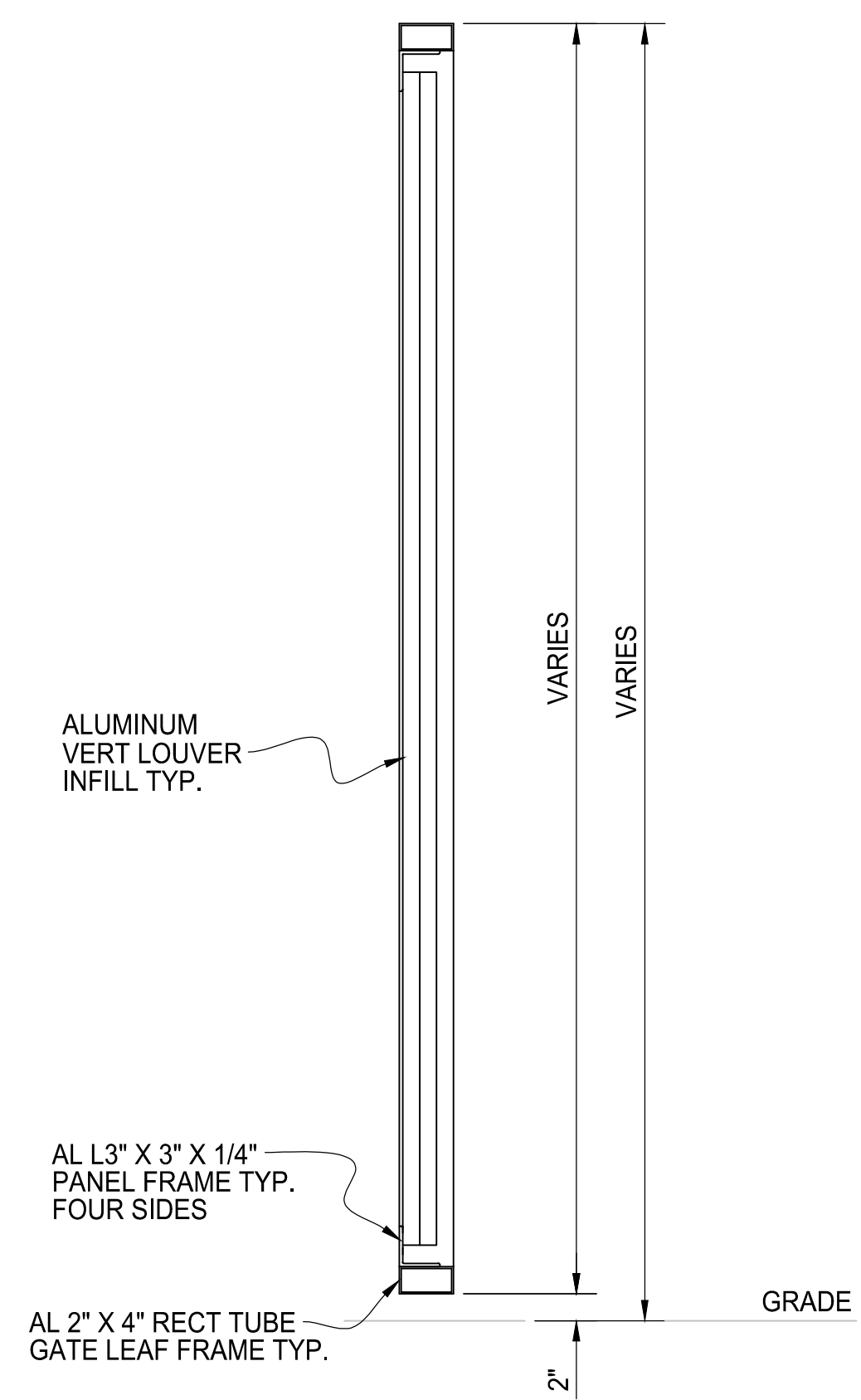
TYPICAL GATE SECTION ALUM 1 3/4\"/>
