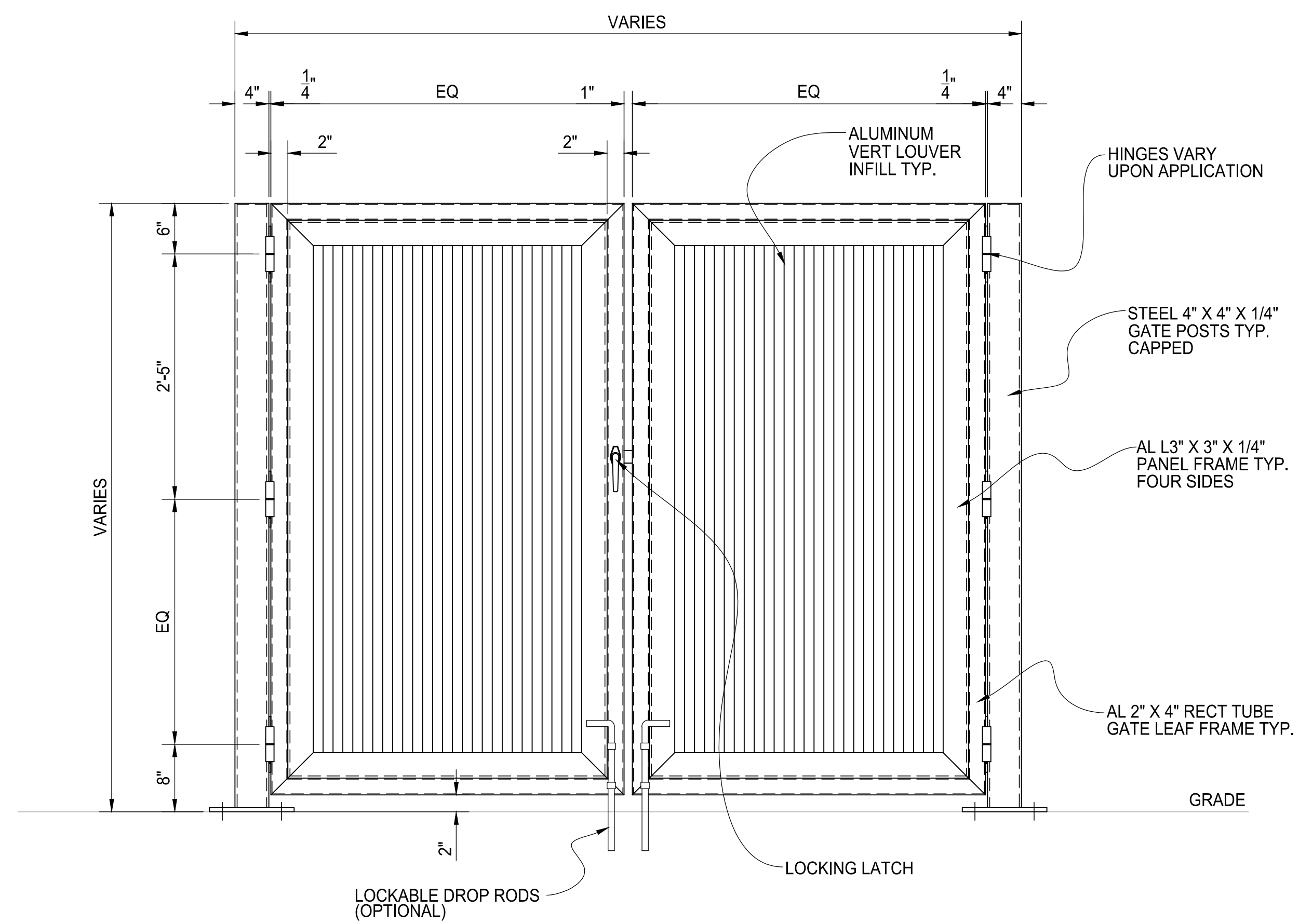
ELEVATION VIEW
