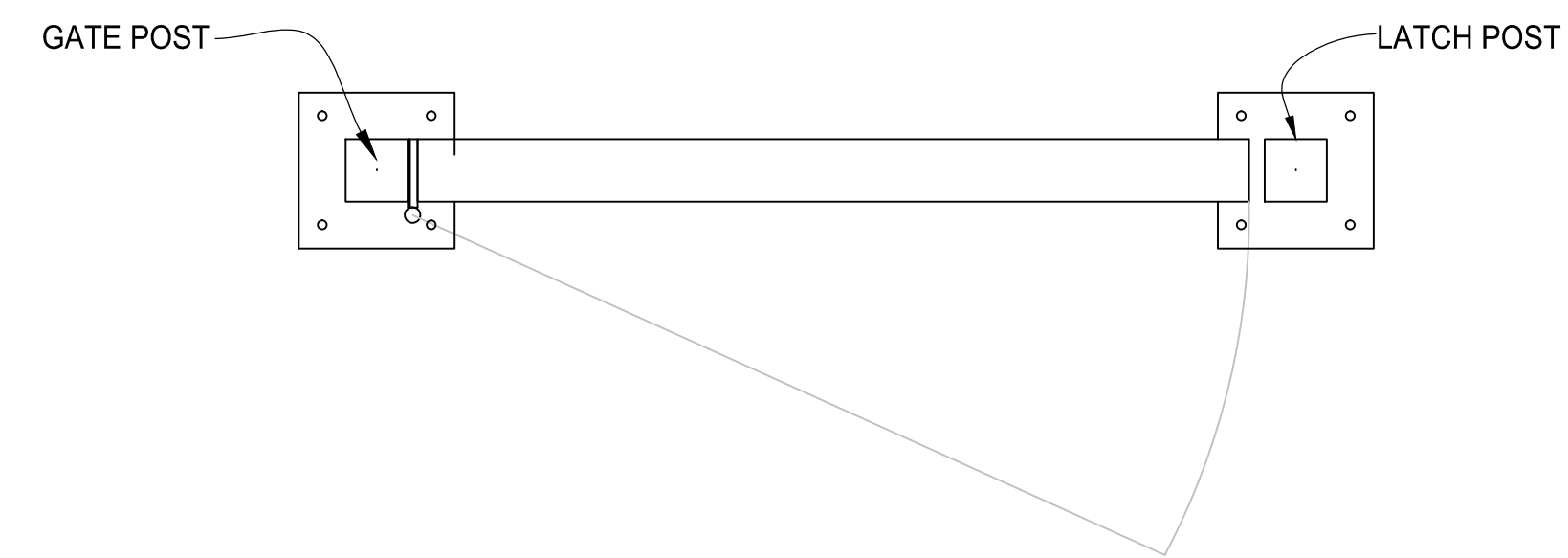
PLAN VIEW
