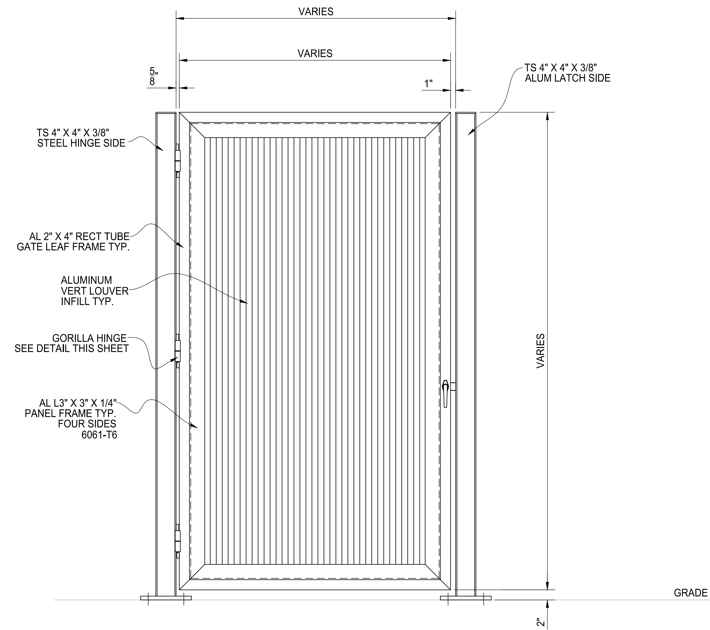
ELEVATION VIEW
