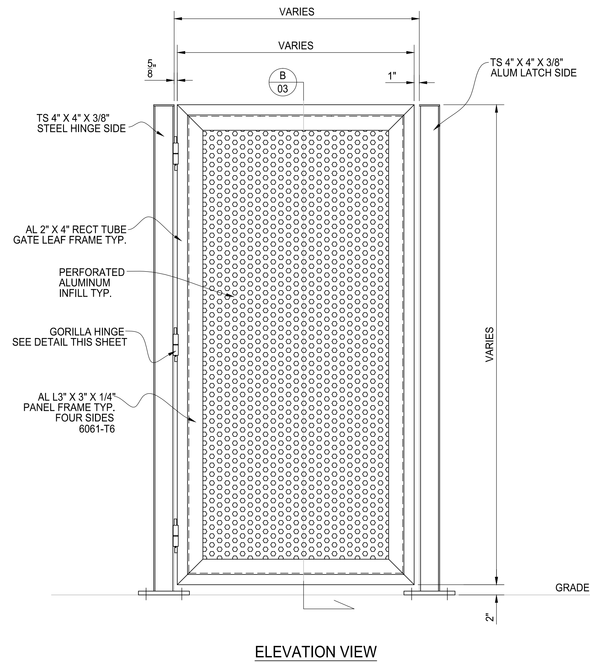
SINGLE SWING GATE ASSEMBLY 1/8" THICK ALUMINUM W/ 1"Ø HOLES ON 1 1/4" CENTERS (58% OPEN)
