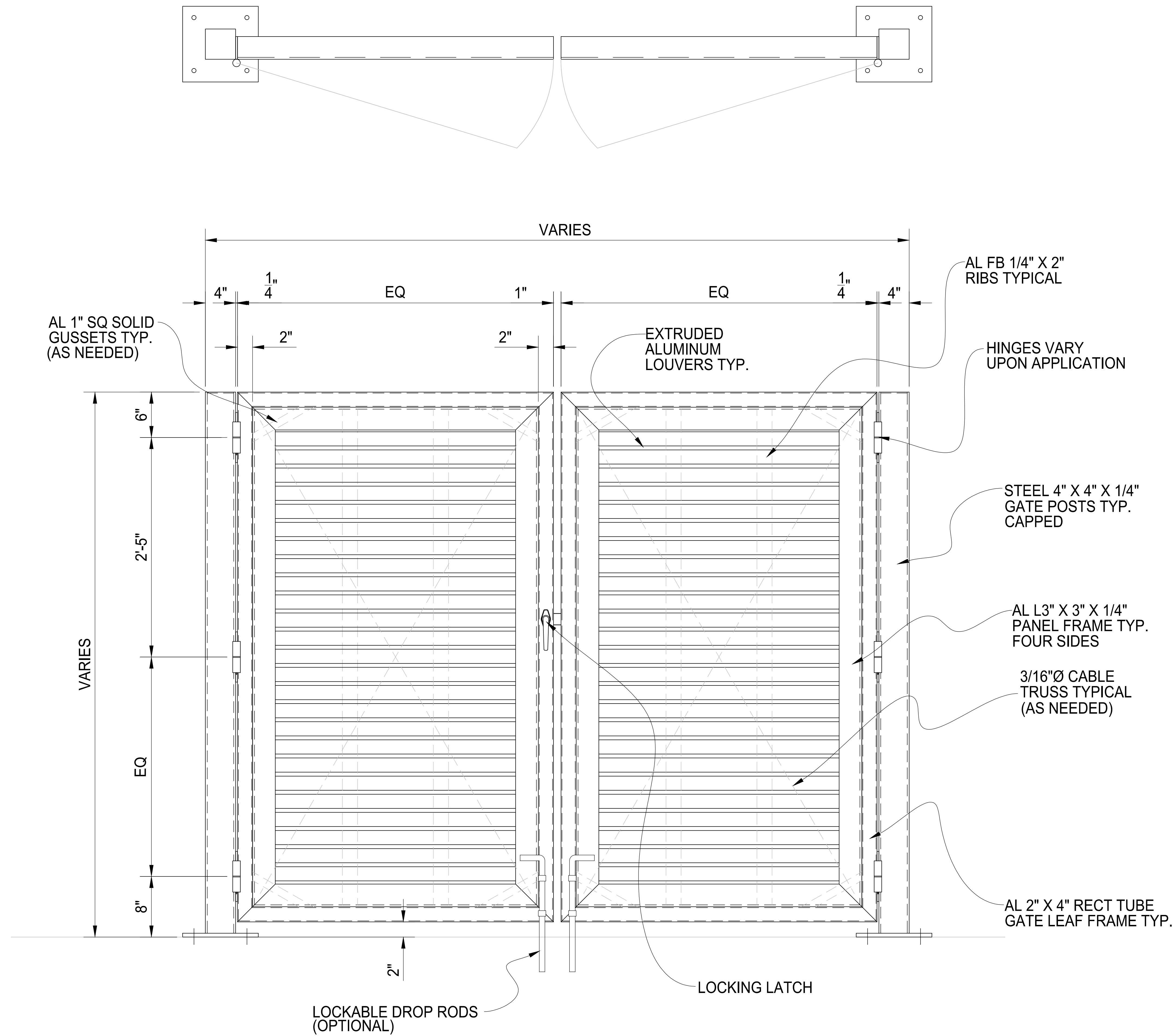
TYPICAL GATE DETAIL
