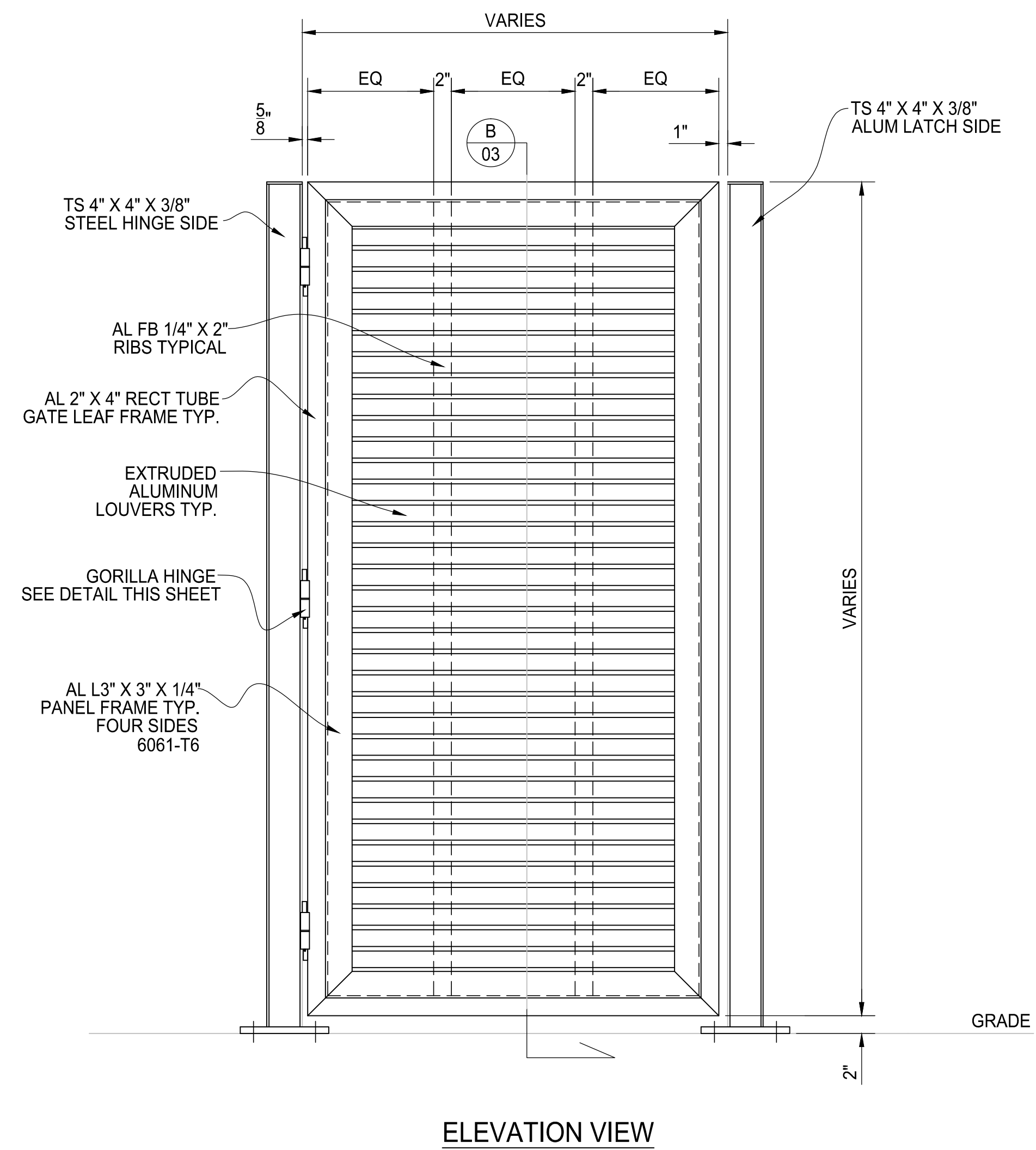
SINGLE SWING GATE ASSEMBLY
