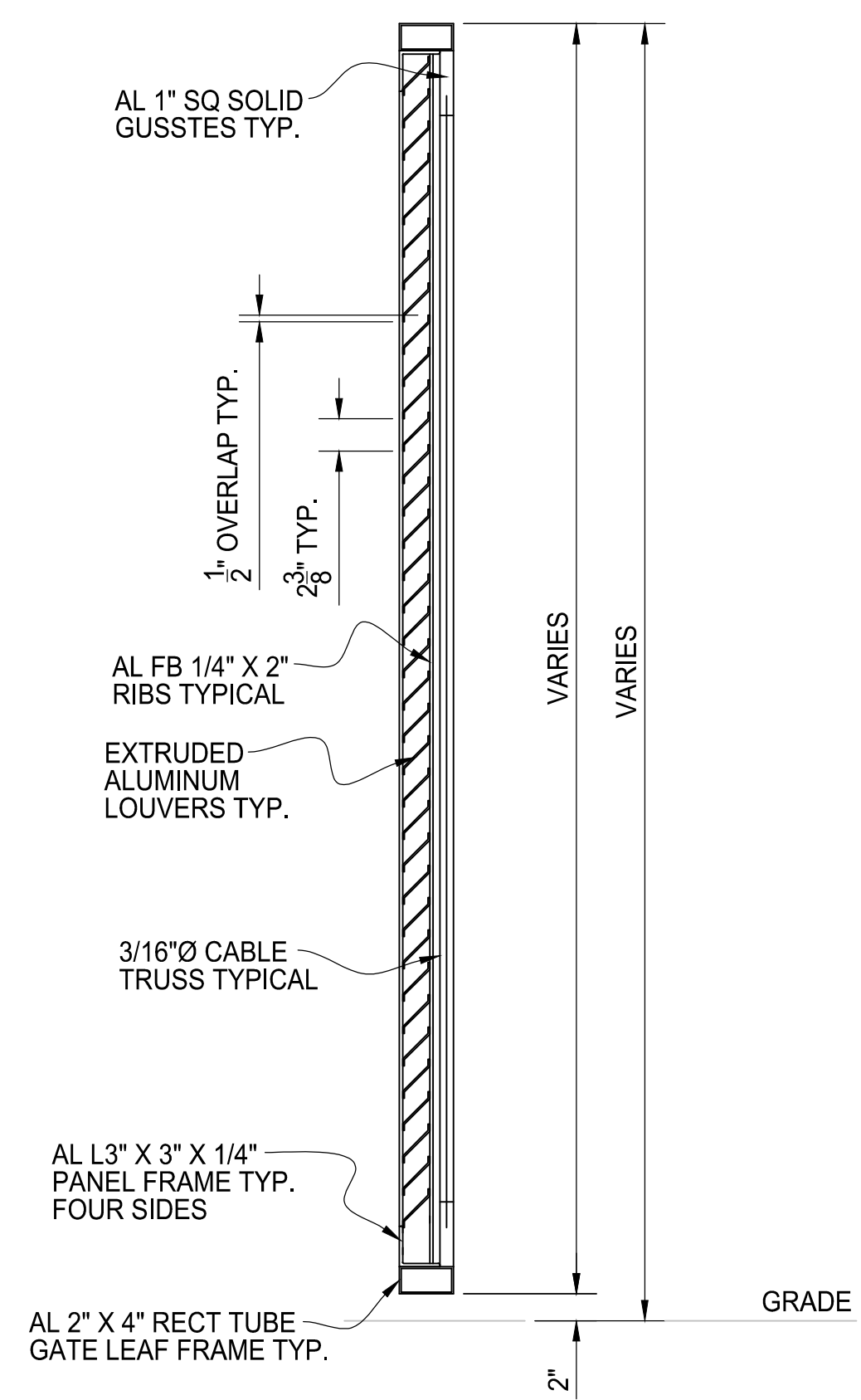
TYPICAL GATE SECTION
