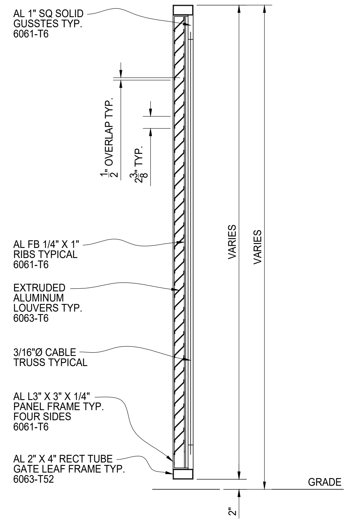
TYPICAL GATE SECTION
