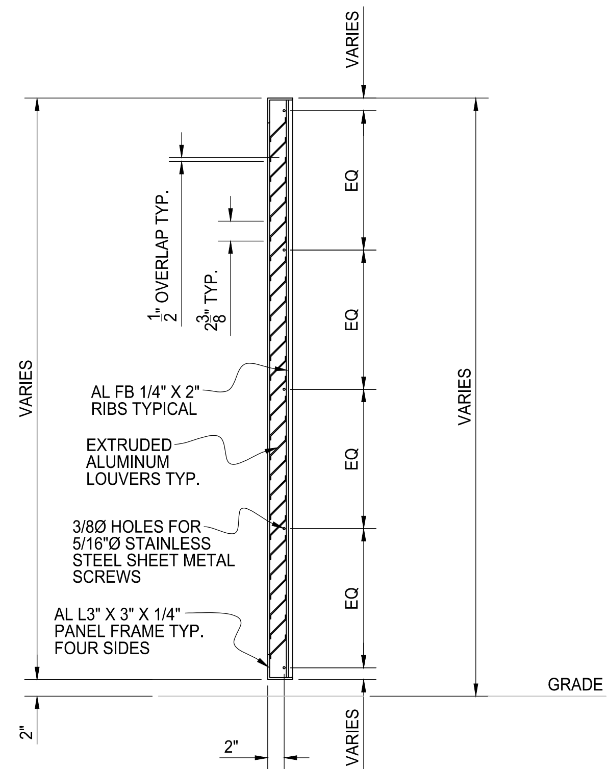
TYPICAL PANEL SECTION
