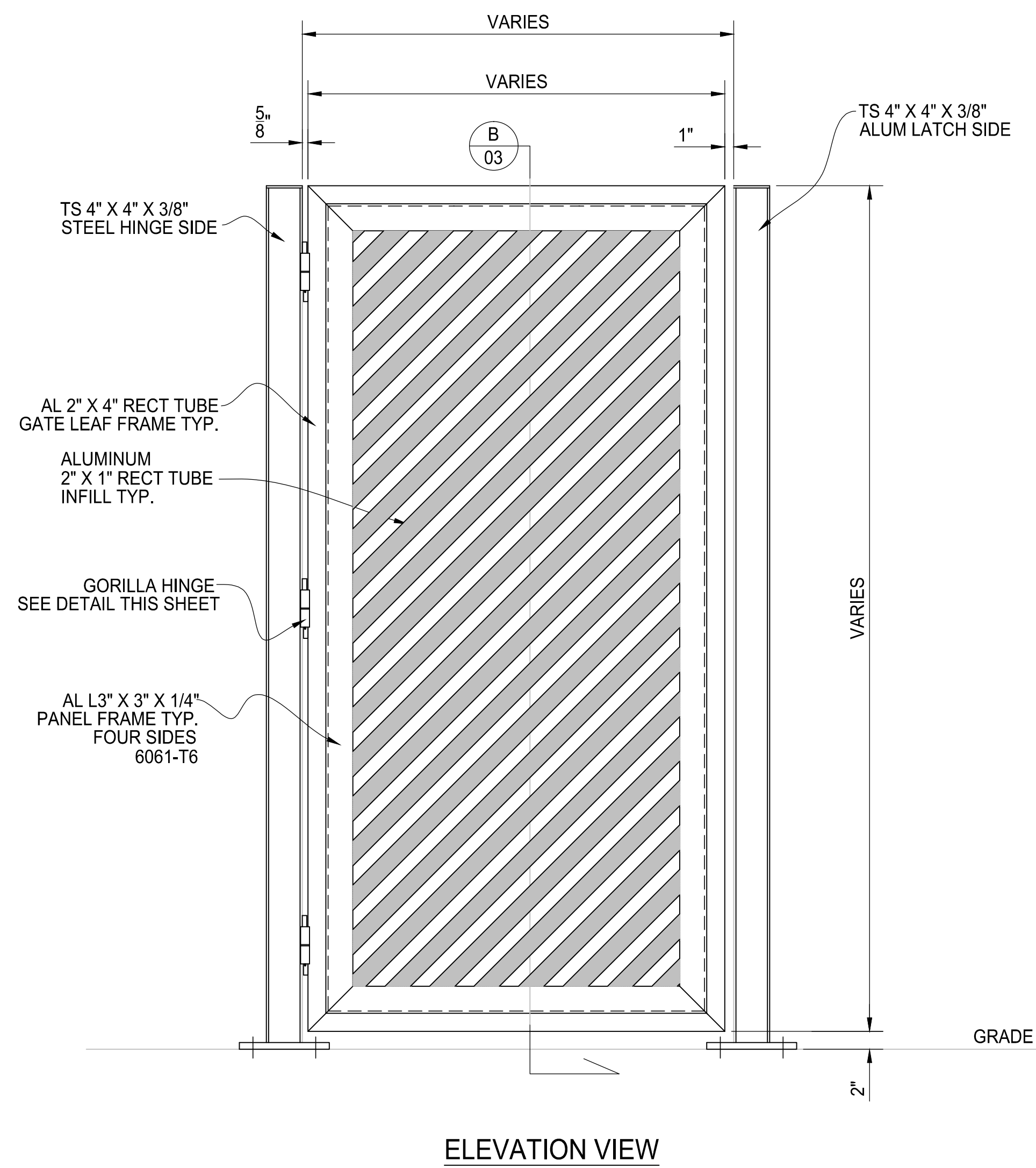
SINGLE SWING GATE ASSEMBLY 2\"/>
