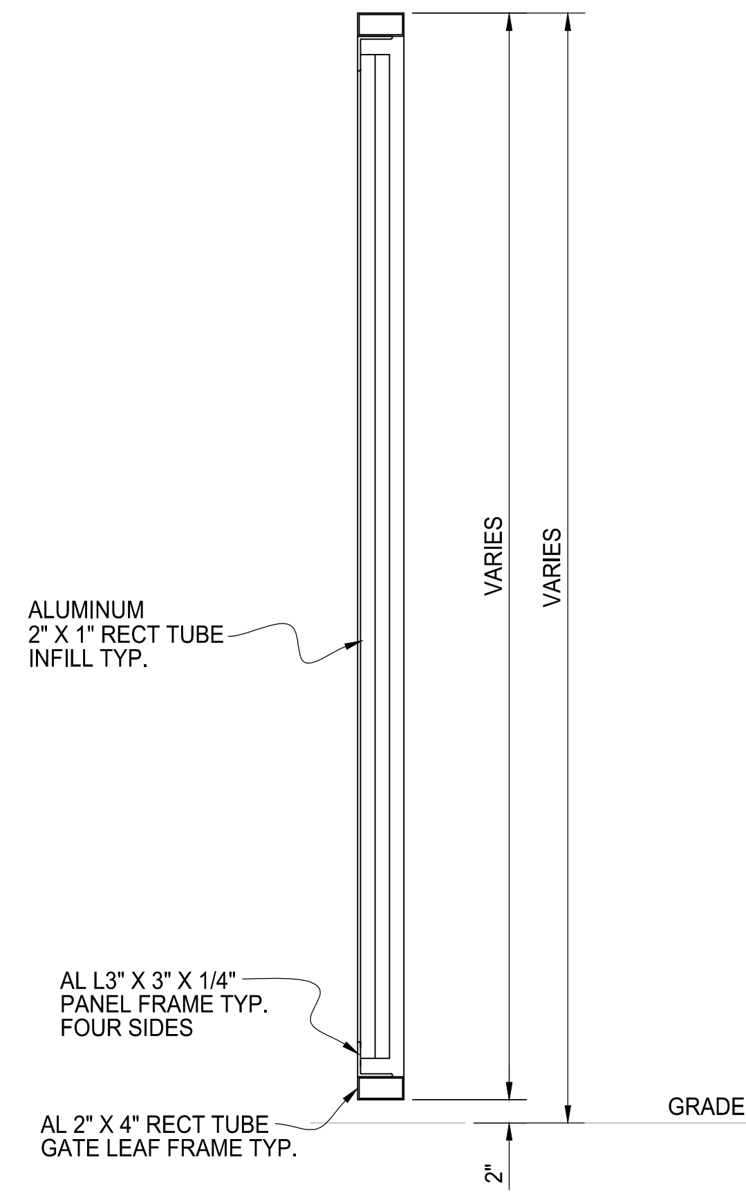
TYPICAL GATE SECTION 2" X 1" ALUM RECT TUBE
