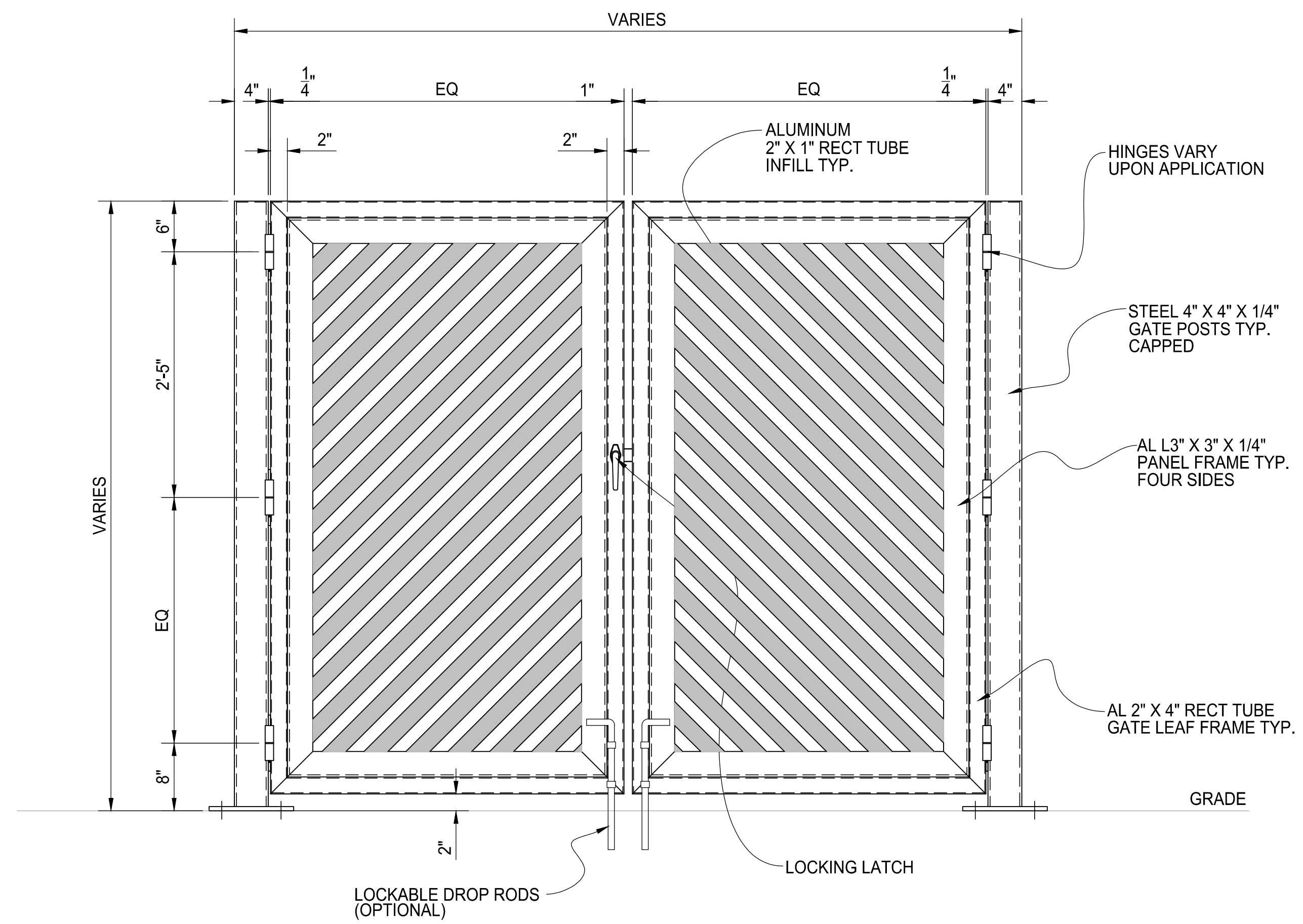
ELEVATION VIEW
