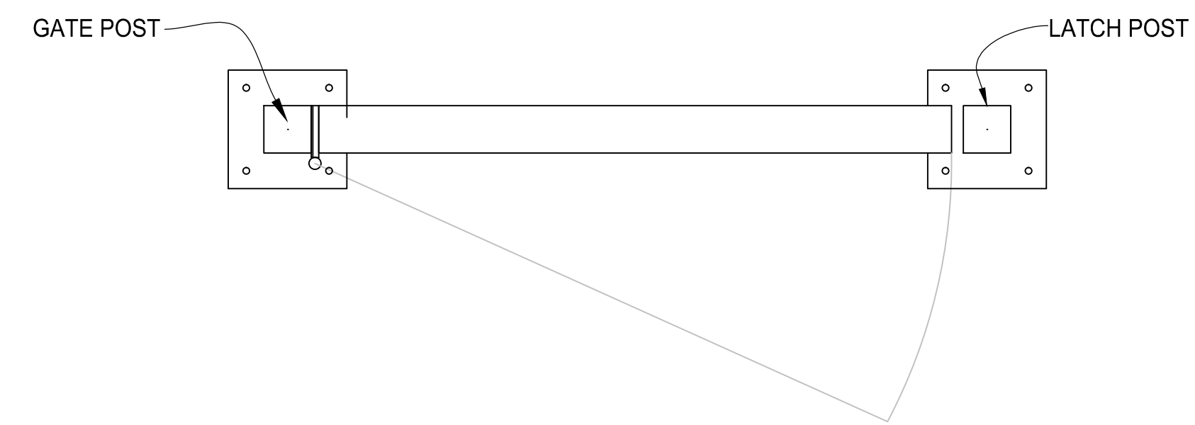
PLAN VIEW
