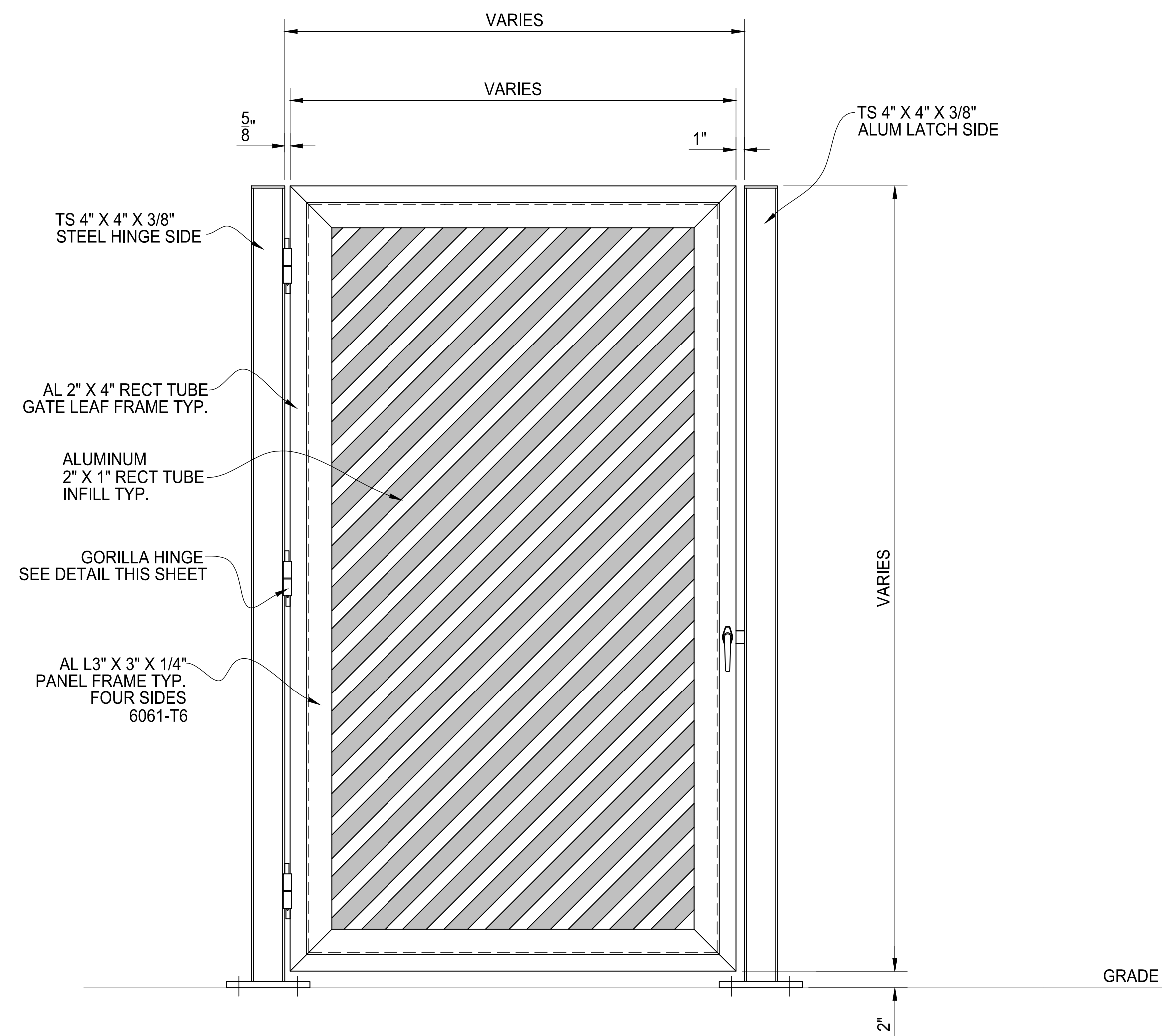
ELEVATION VIEW
