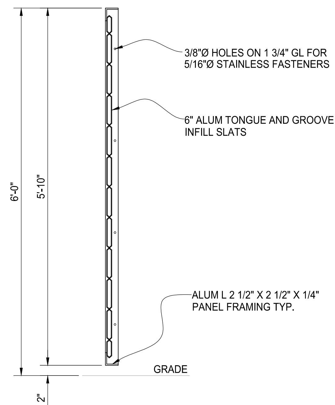
TYPICAL PANEL SECTION
