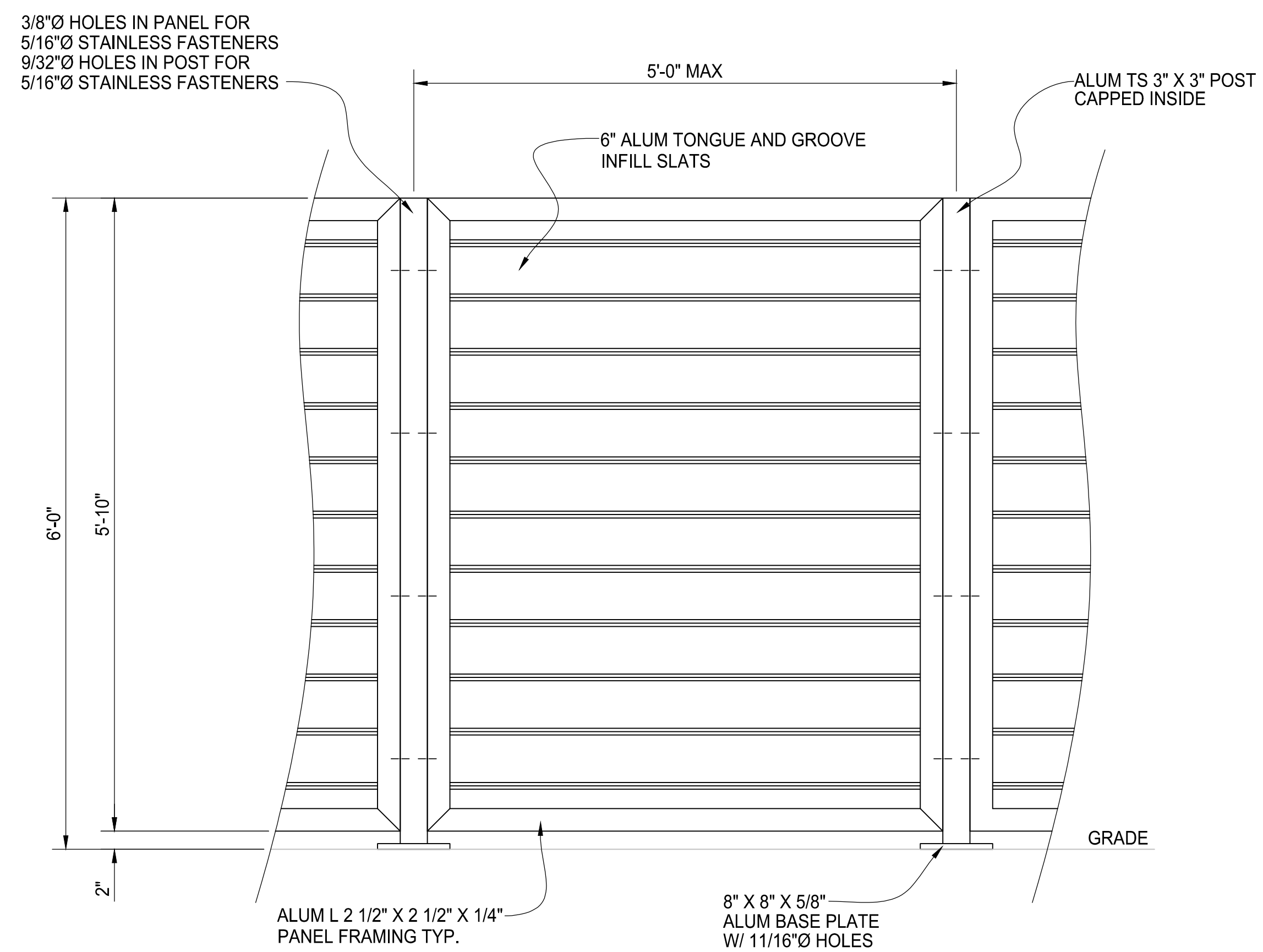
TYPICAL PANEL/POST DETAIL
