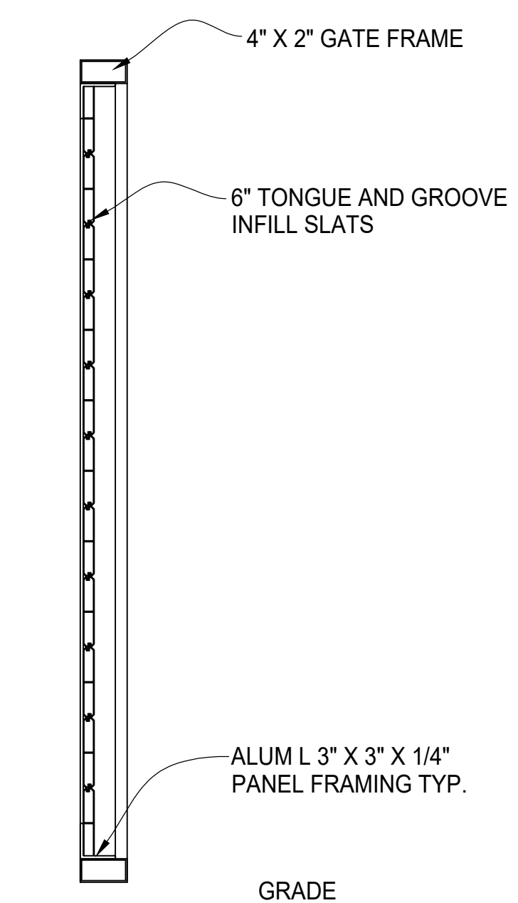
TYPICAL GATE SECTION
