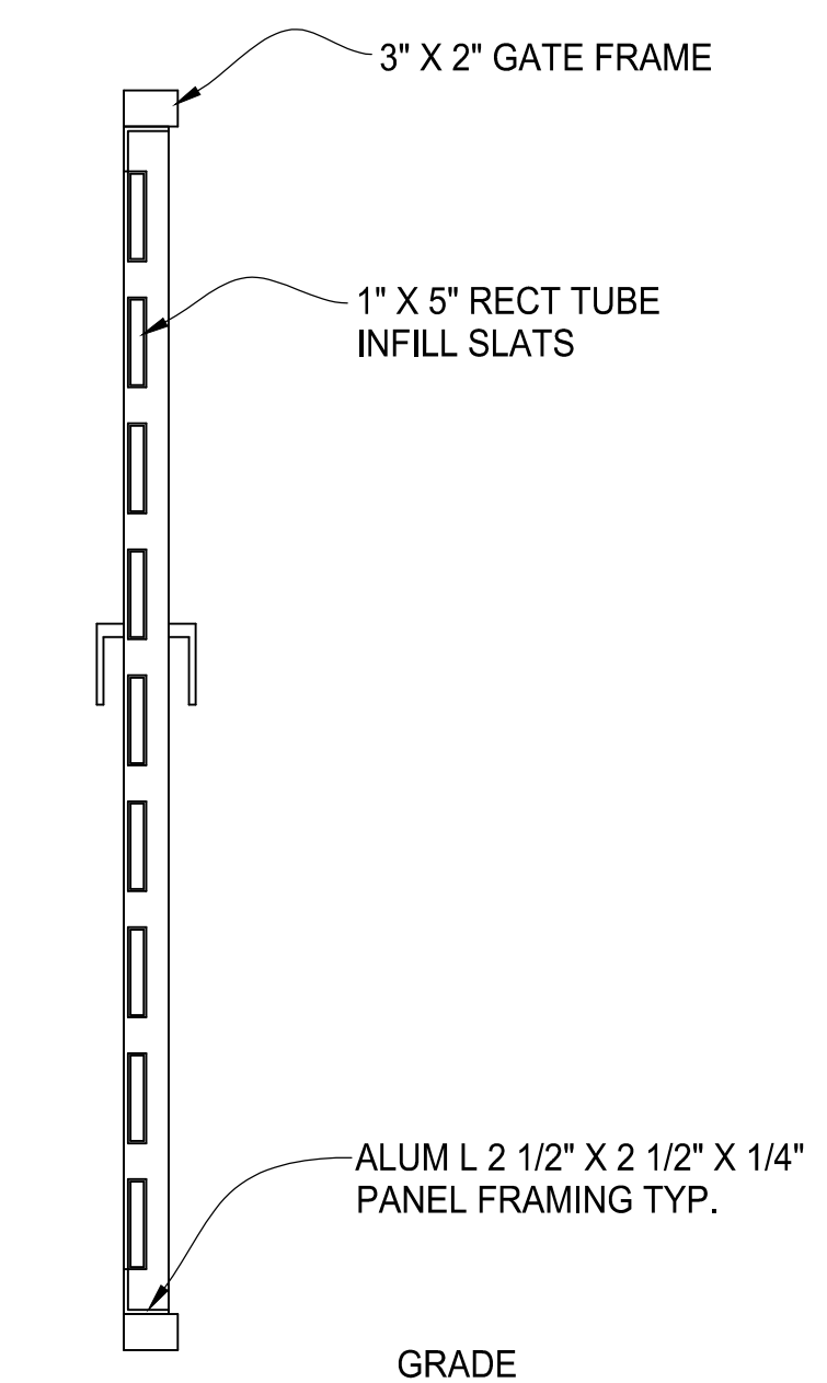
TYPICAL GATE SECTION
