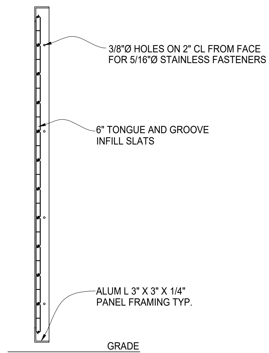
TYPICAL GATE SECTION
