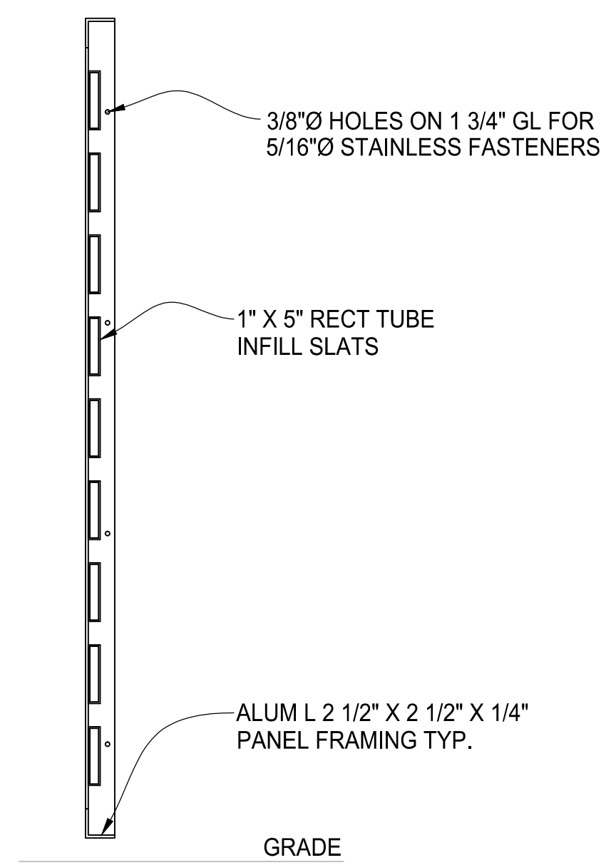
TYPICAL GATE SECTION
