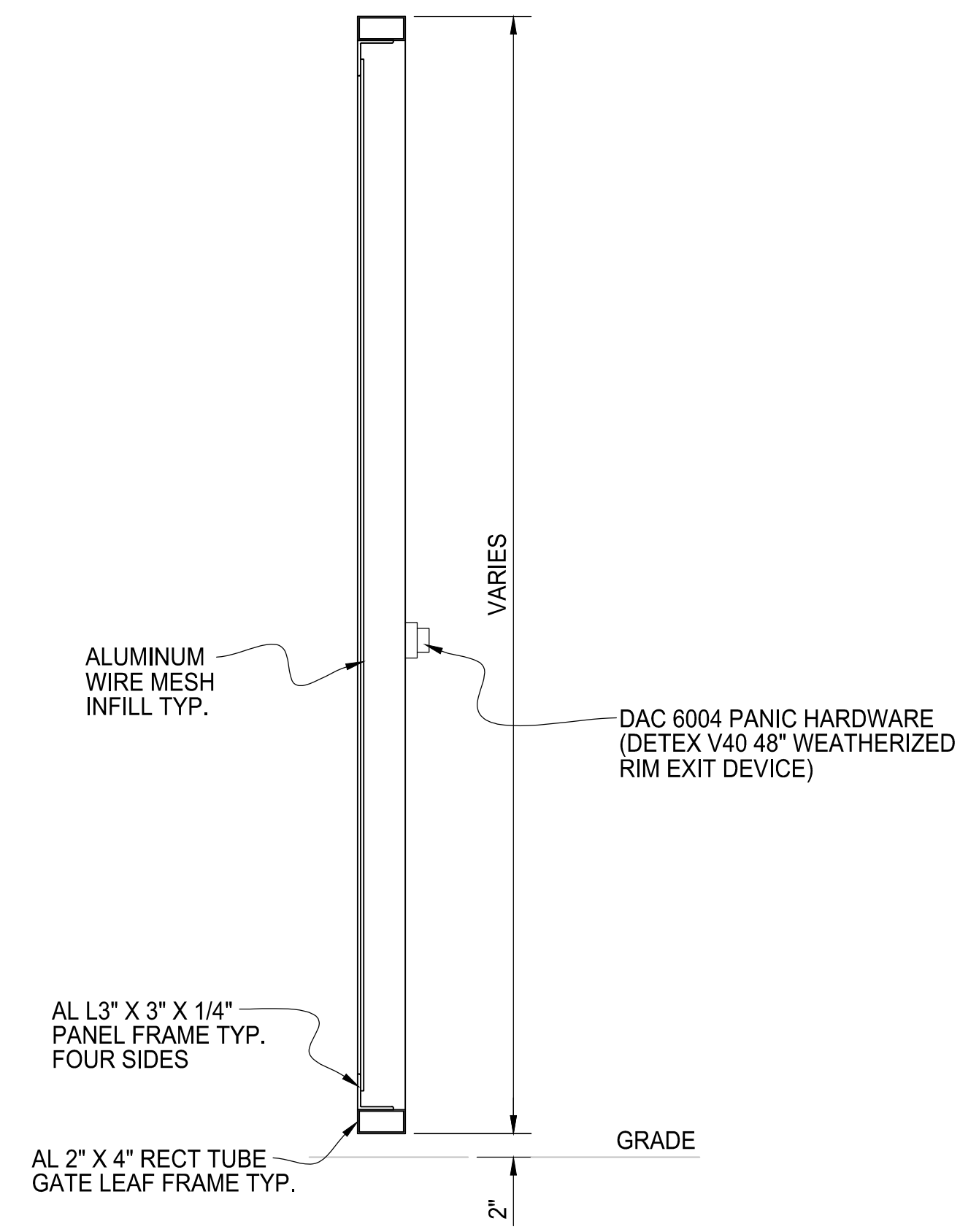
B TYPICAL GATE SECTION
