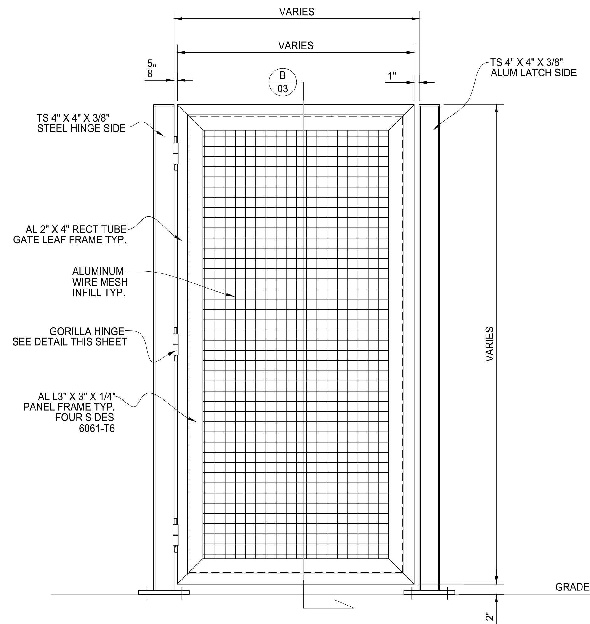
ELEVATION VIEW
