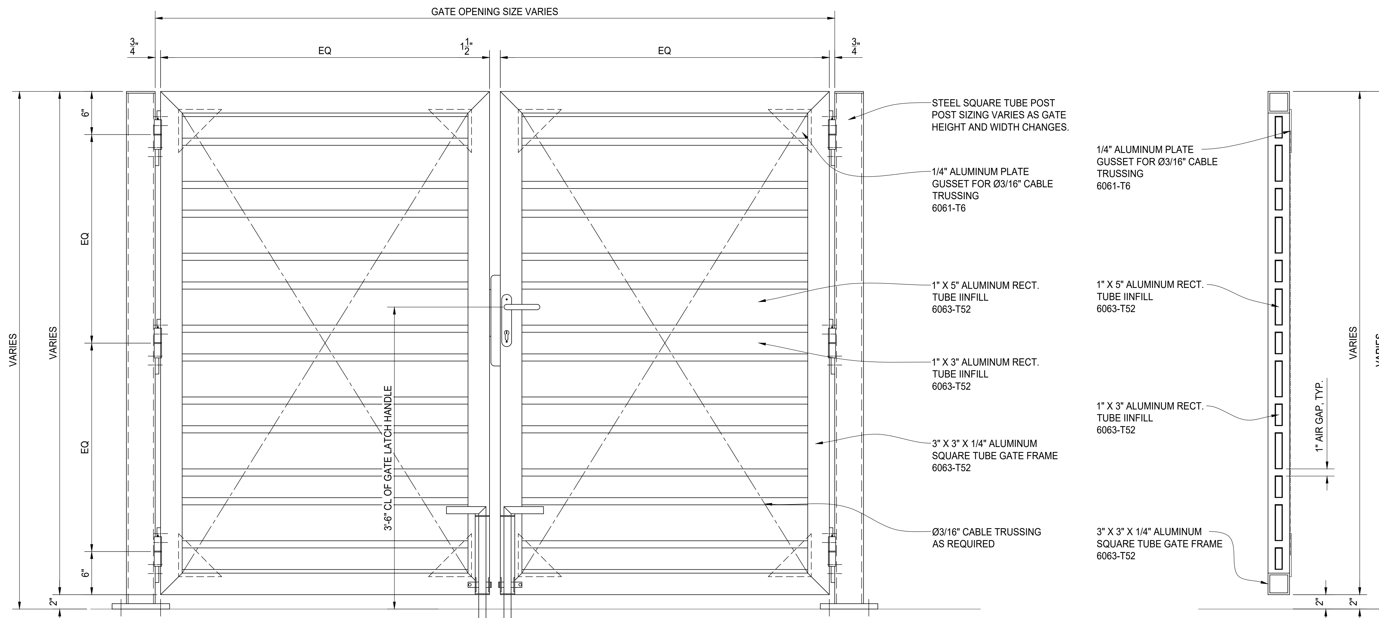
GATE ELEVATION
