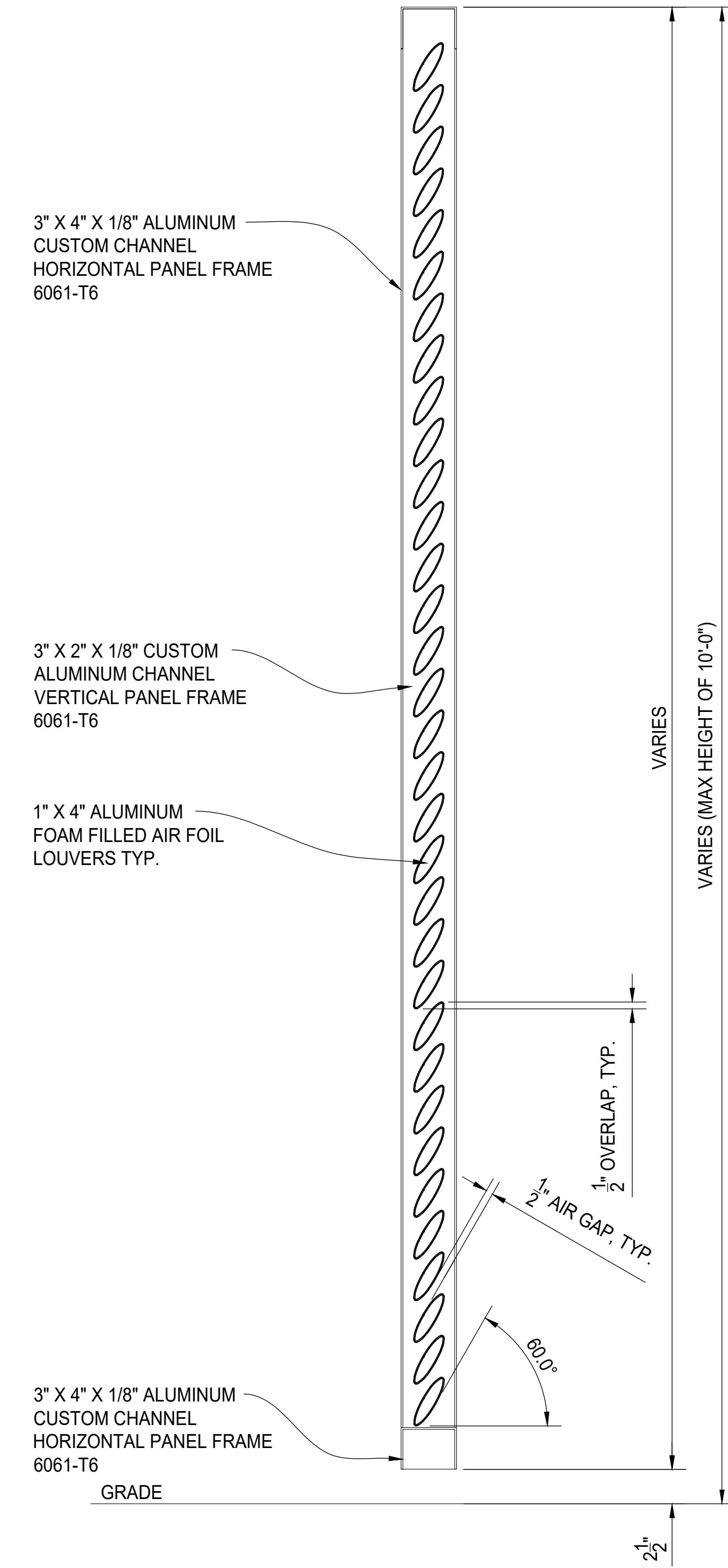
TYPICAL PANEL SECTION
