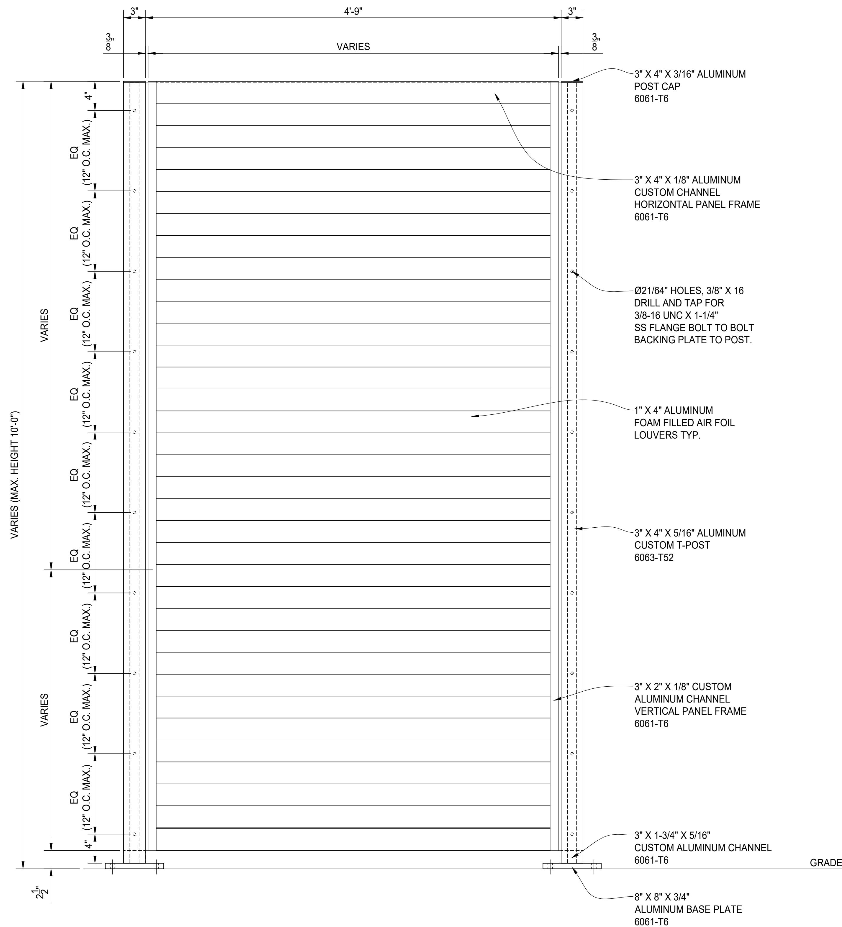
PANEL ELEVATION
